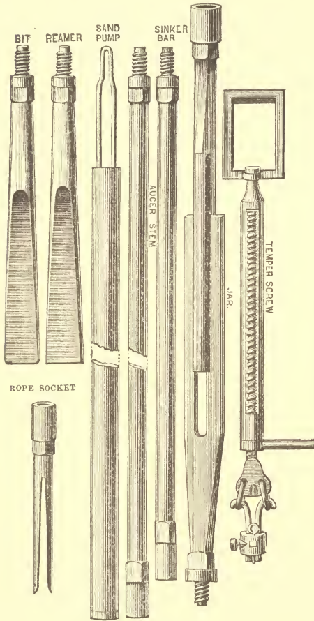
Boring Tools.
